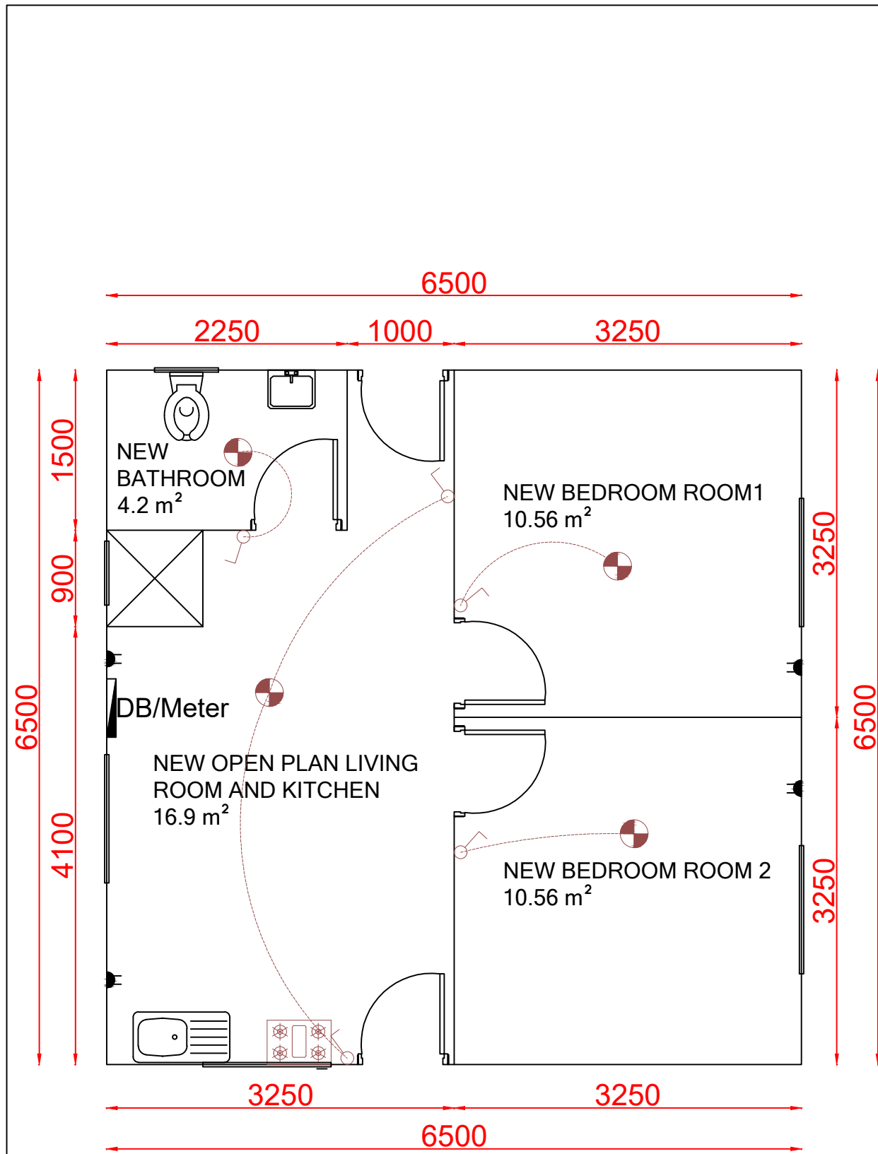
2 BEDROOM FLOOR AND ELETRICAL LAYOUT
