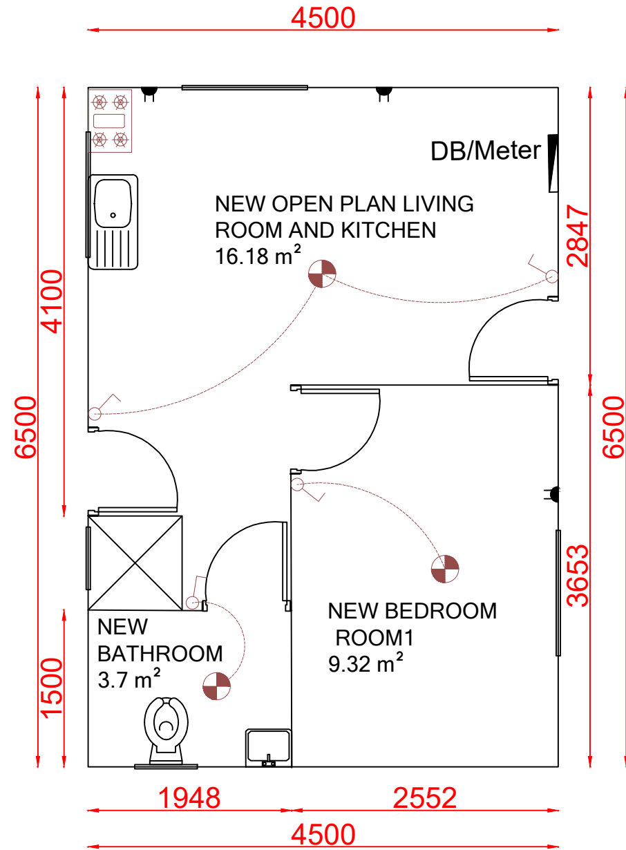
1 BEDROOM FLOOR AND ELETRICAL LAYOUT
